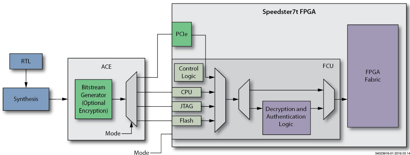
Figure 13: Bitstream Generation and Configuration Process
