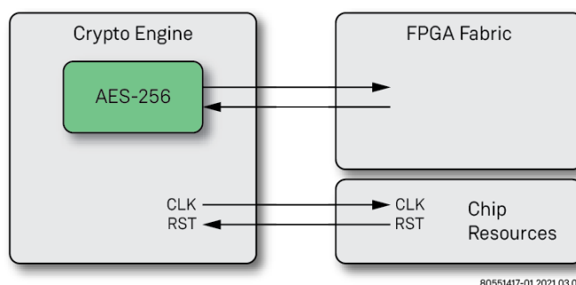
Figure 11: The Speedster Cryptographic Engine
