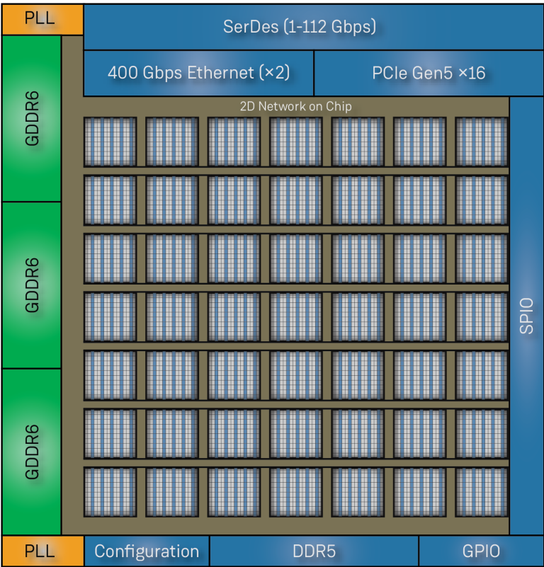
Figure 2: AC7t800 Top-Level Block Diagram
