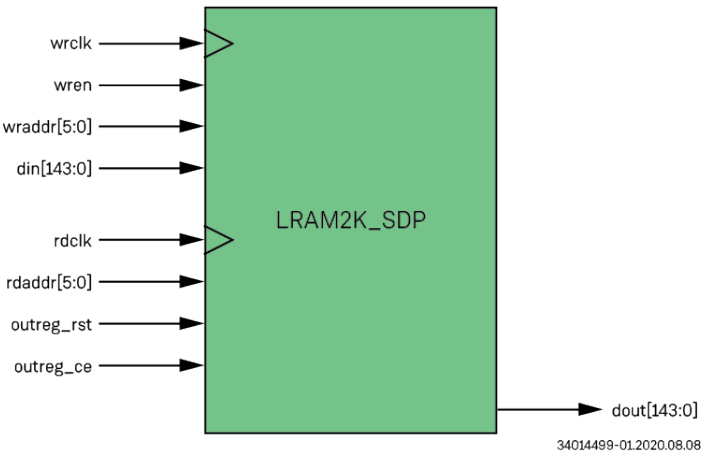
Figure 8: LRAM2K Block Diagram
