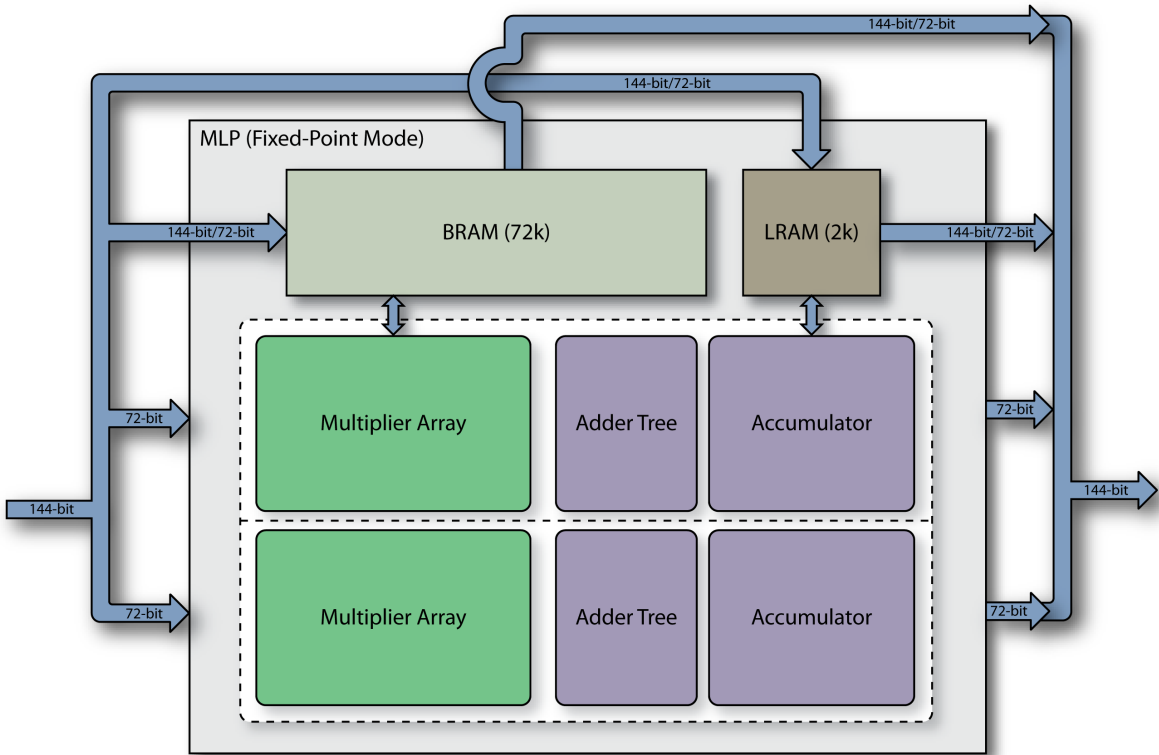
Figure 4: MLP Using Fixed-Point Mode
