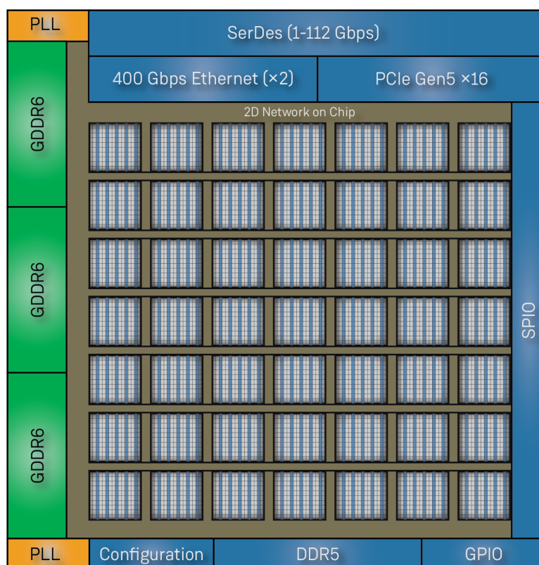
Figure 10: Speedcore7t AC7t800 NoC
