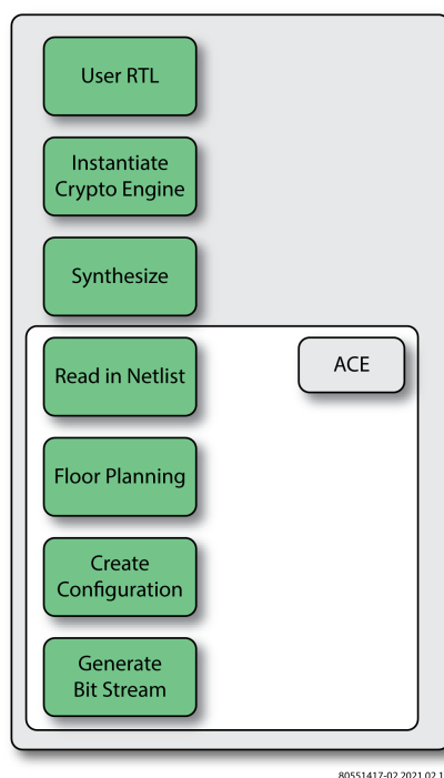
Figure 12: Design Flow for the Speedster Cryptographic Engine
