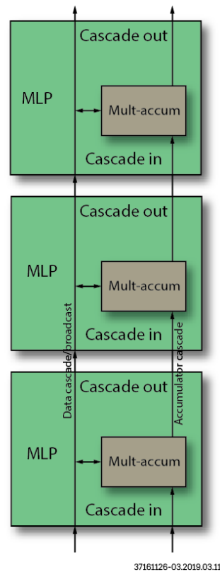
Figure 6: MLP Cascade Path
