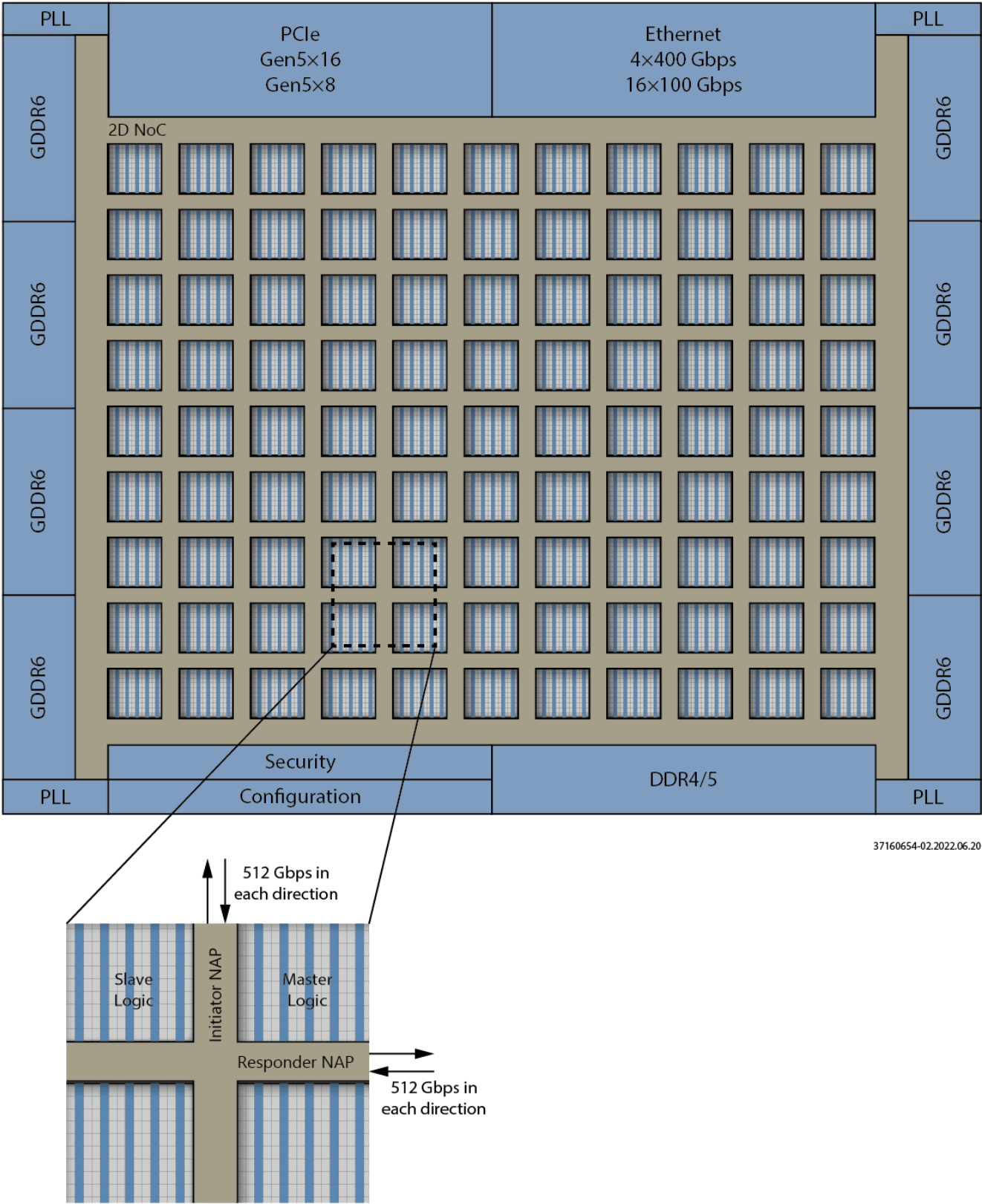
Figure 9: Speedcore7t AC7t1500 NoC Showing Initiator and Responder Endpoints
