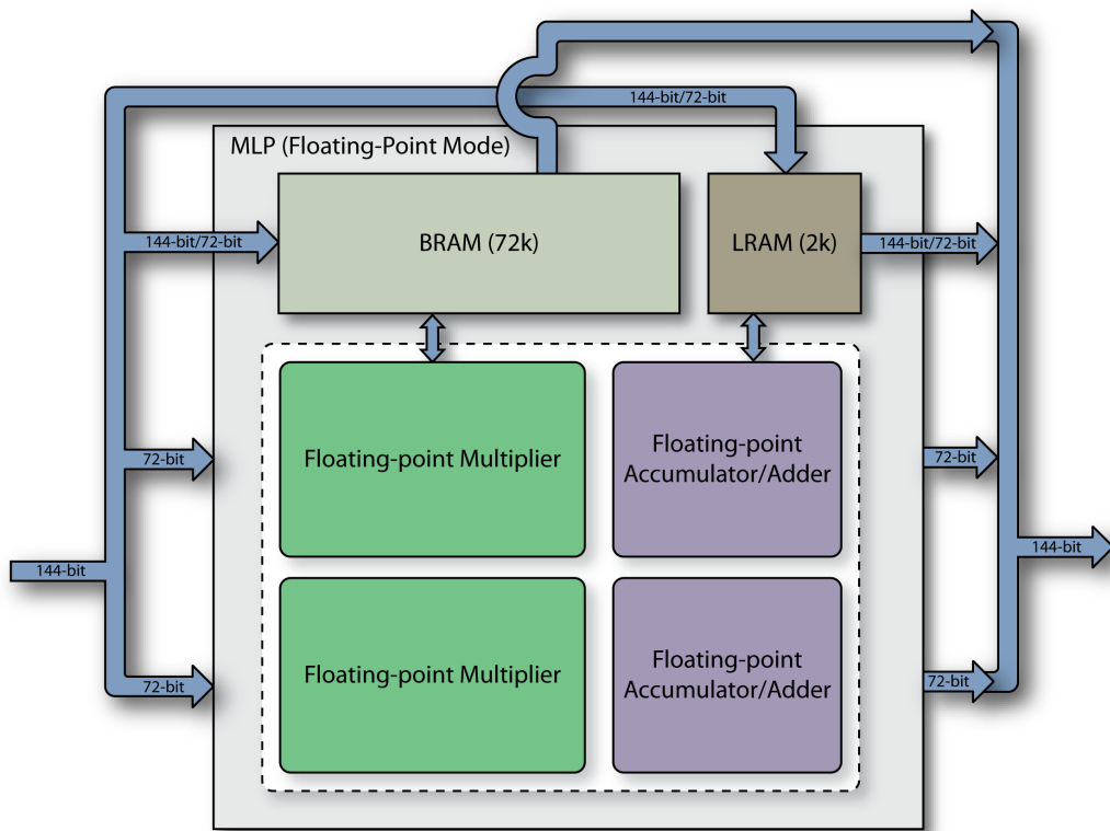
Figure 5: MLP Using Floating-Point Mode
