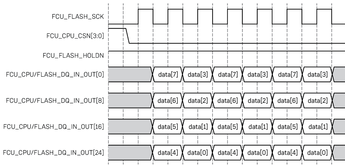
Figure 12 • 4D Flash SPI Read Data Ordering
