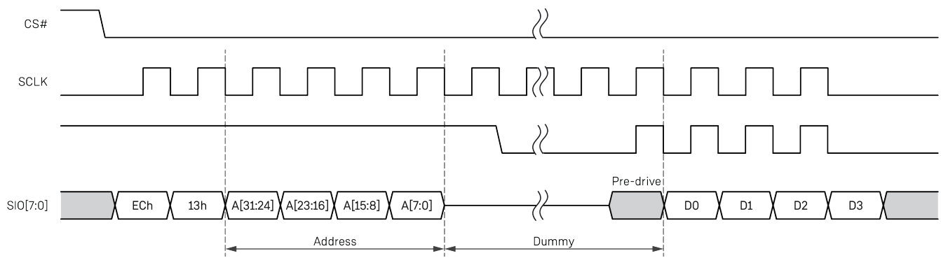
Figure 17 • Octa Read Mode (8READ) Timing
