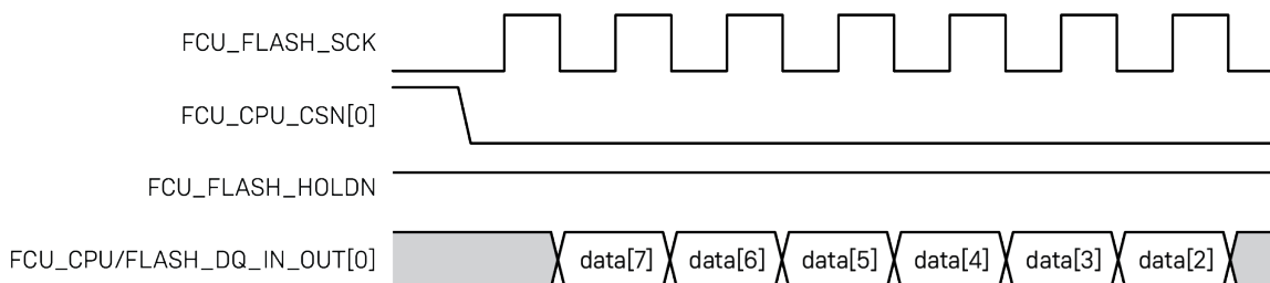
Figure 9 • Speedster7t FPGA 1D Octa Mode Flash Programming Configuration
