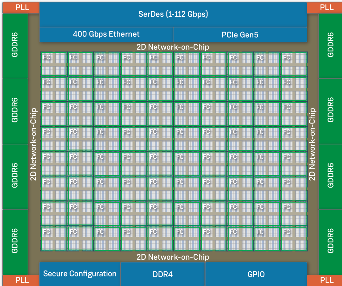
Figure 61 • AC7t1500 FPGA Partial Reconfiguration Fabric Cluster Layout
