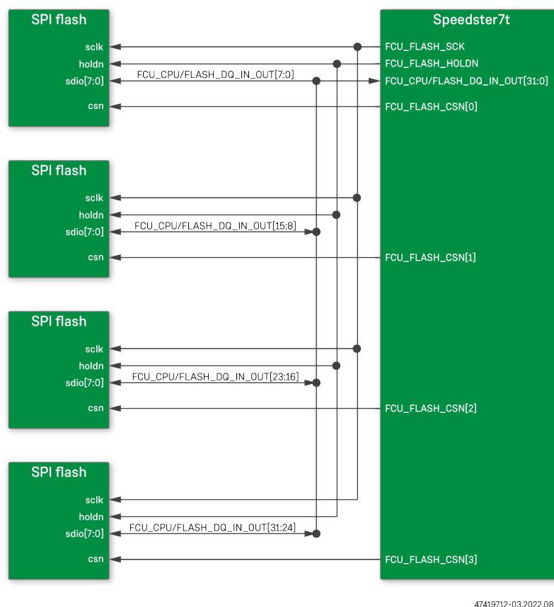
Figure 11 • Speedster7t FPGA 4D Flash Programming Configuration
