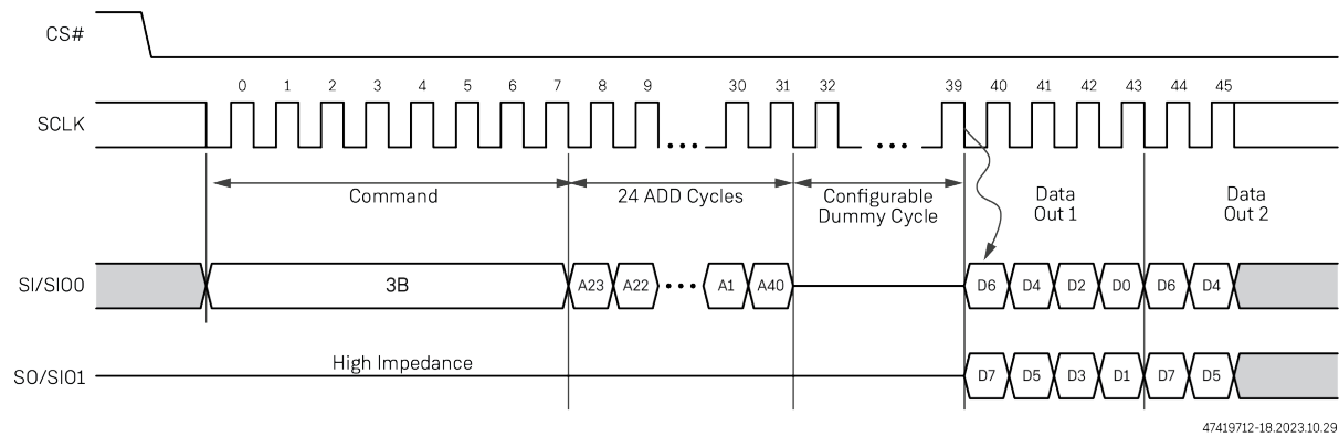
Figure 15 • Dual Read Mode (DREAD) Timing
