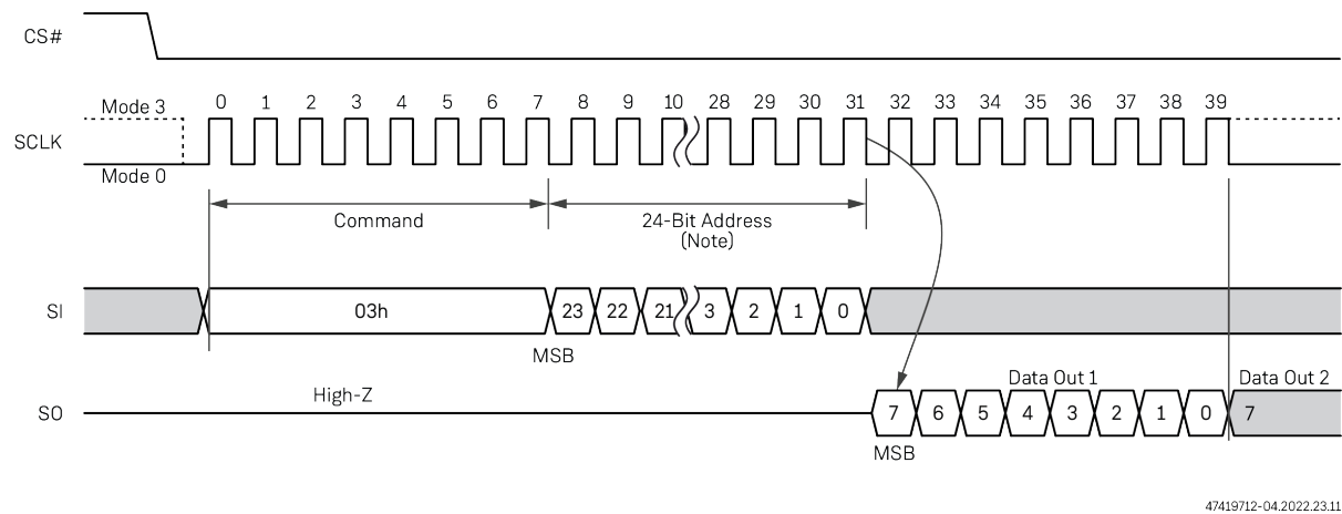
Figure 14 • SPI Read Mode Timing
