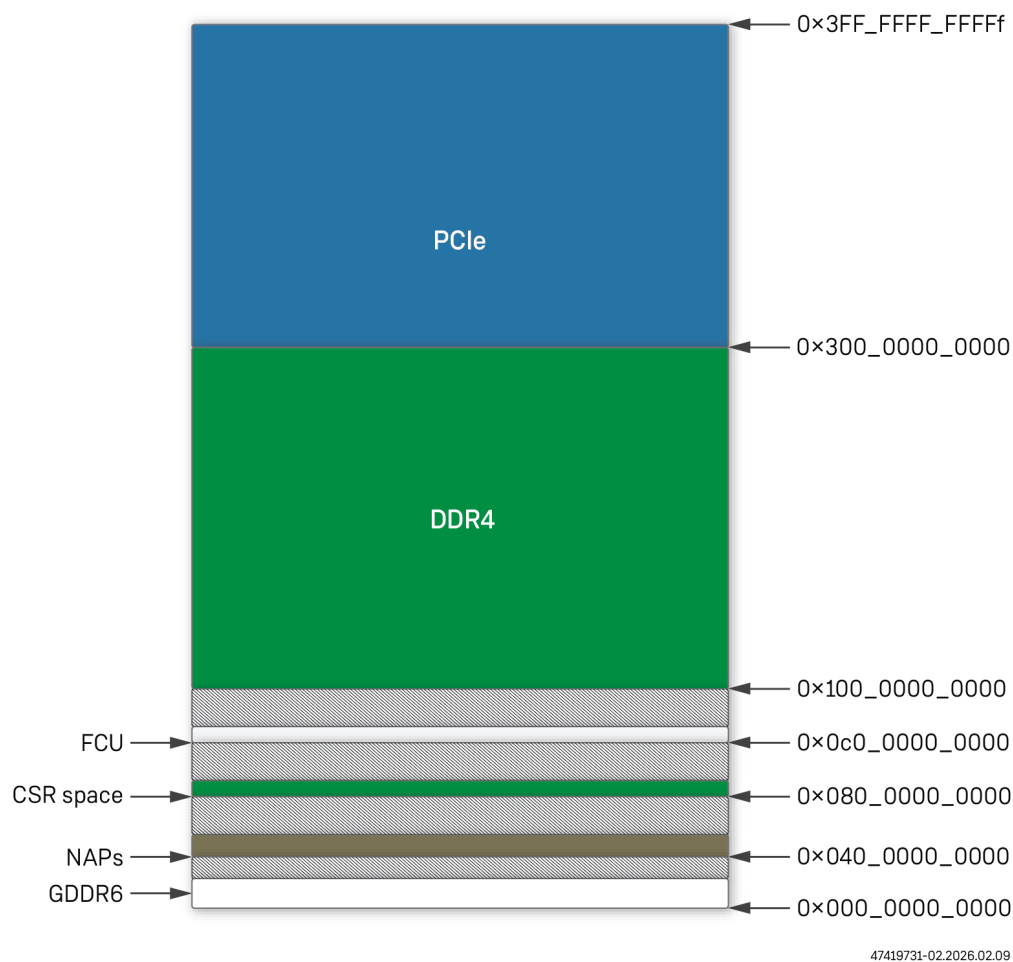
Figure 19 · 2D NoC Address Space for AC7t800
