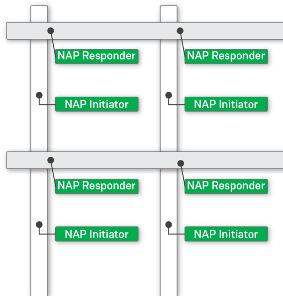
Figure 6 • NoC Access Points in FPGA Fabric
