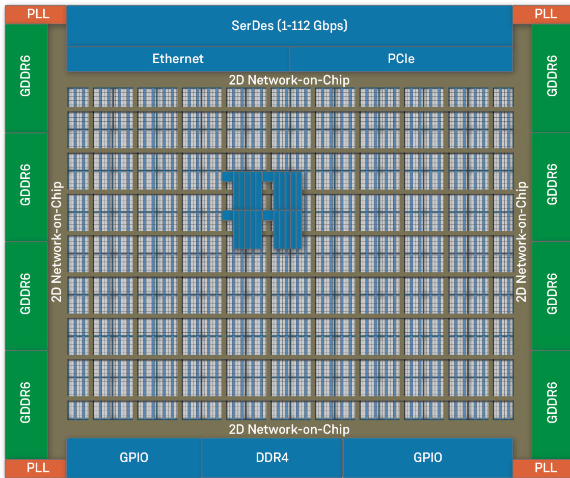
Figure 15 • Quad-Segmented Mode on the 2D NoC
