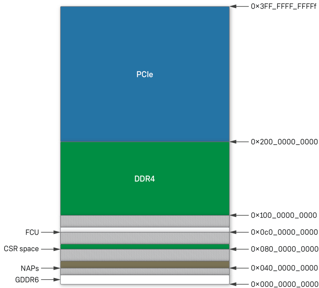
Figure 18 • 2D NoC Address Space for AC7t1500
