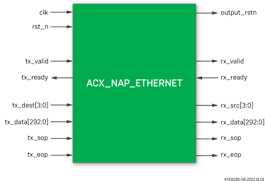
Figure 11 • Ethernet NAP Block Diagram
