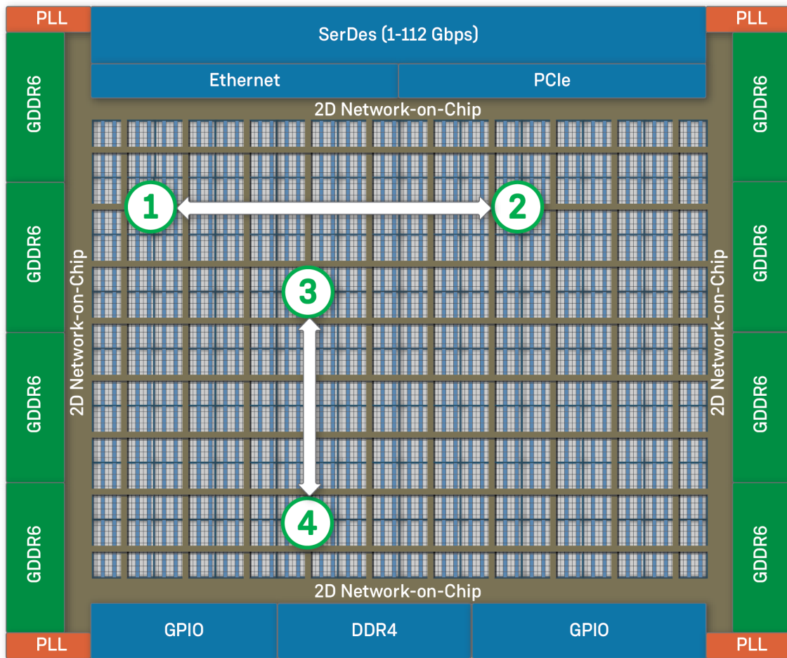
Figure 17 • Data Streaming
