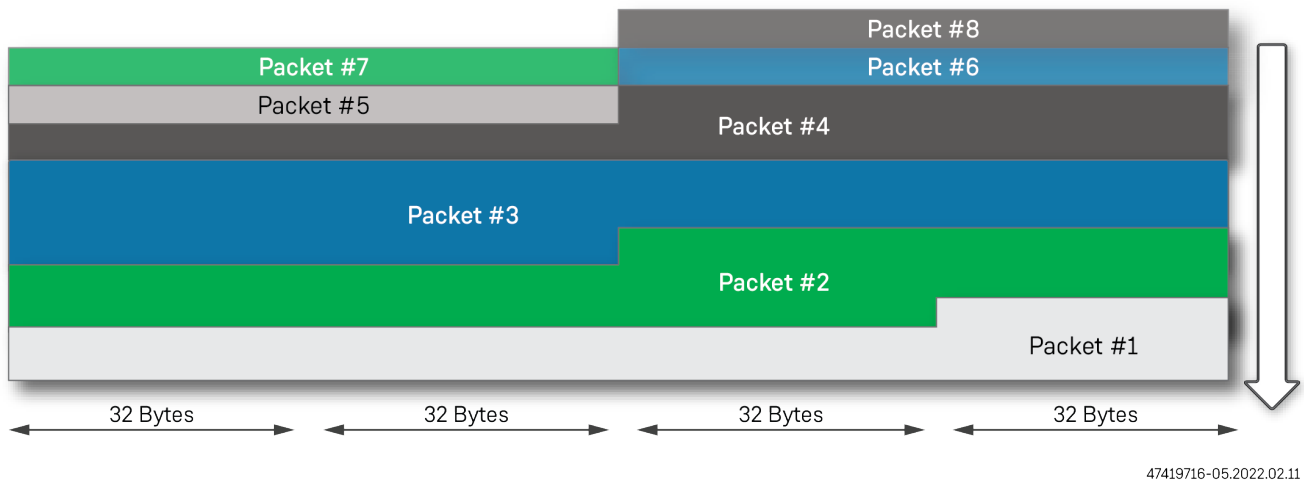
Figure 14 • Packet Segmentation for Quad-Segmented Mode
