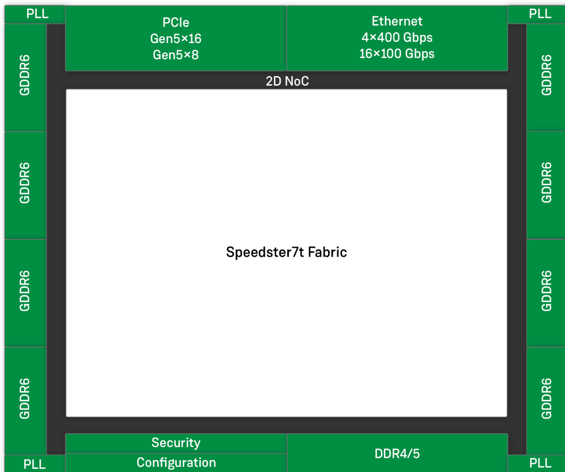
Figure 2 • Speedster7t 2D NoC Peripheral Ring
