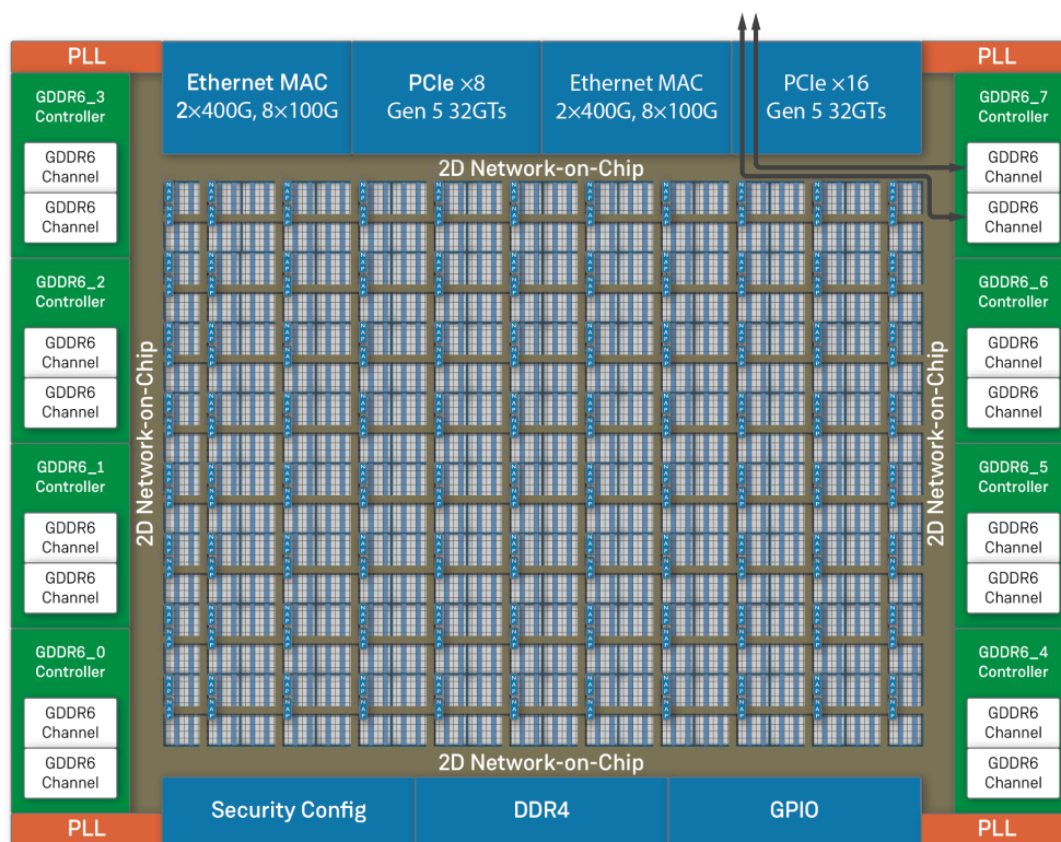
Figure 12 • PCIe-to-GDDR6 Transactions
