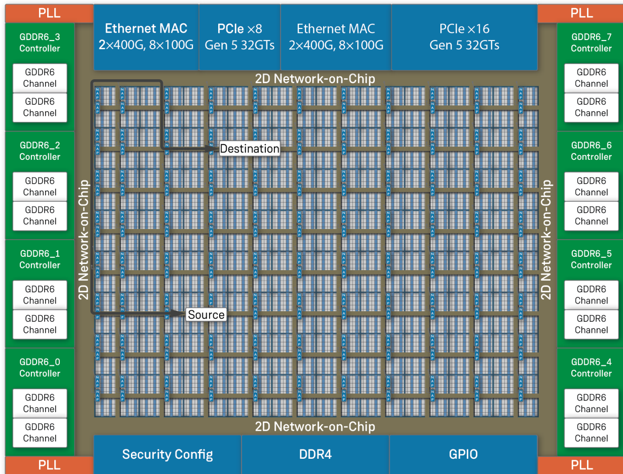
Figure 16 • AXI Mode Fabric-to-Fabric Transaction
