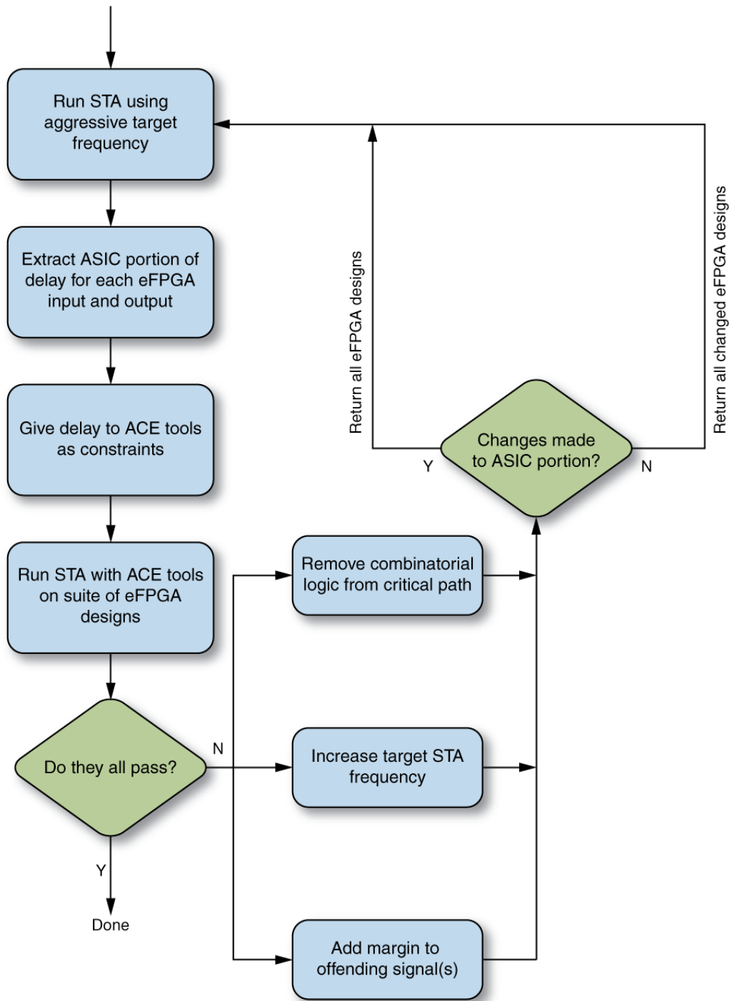
Figure 3: Timing Closure in the Advanced Mode
