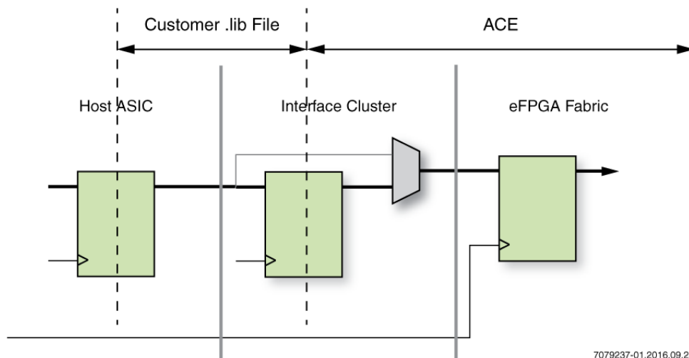
Figure 1: Simple Timing Mode
