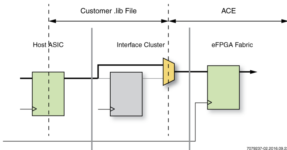
Figure 2: Advanced Timing Mode
