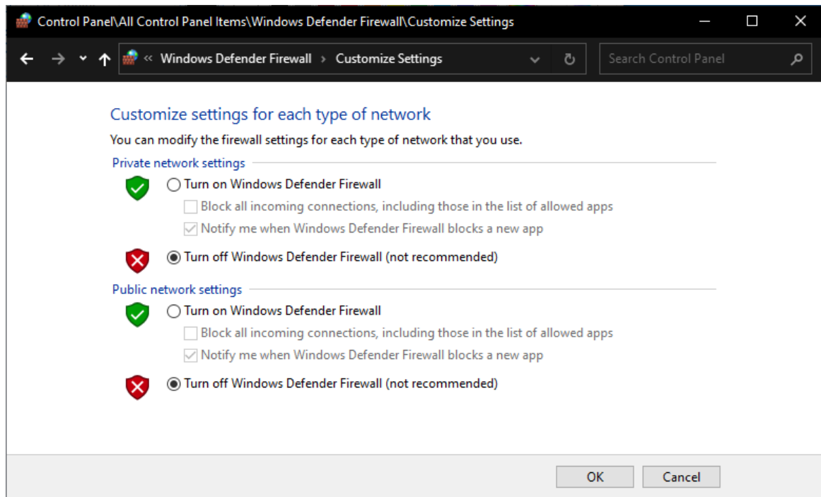
Figure 58: Windows Defender Firewall Customize Settings Dialog
