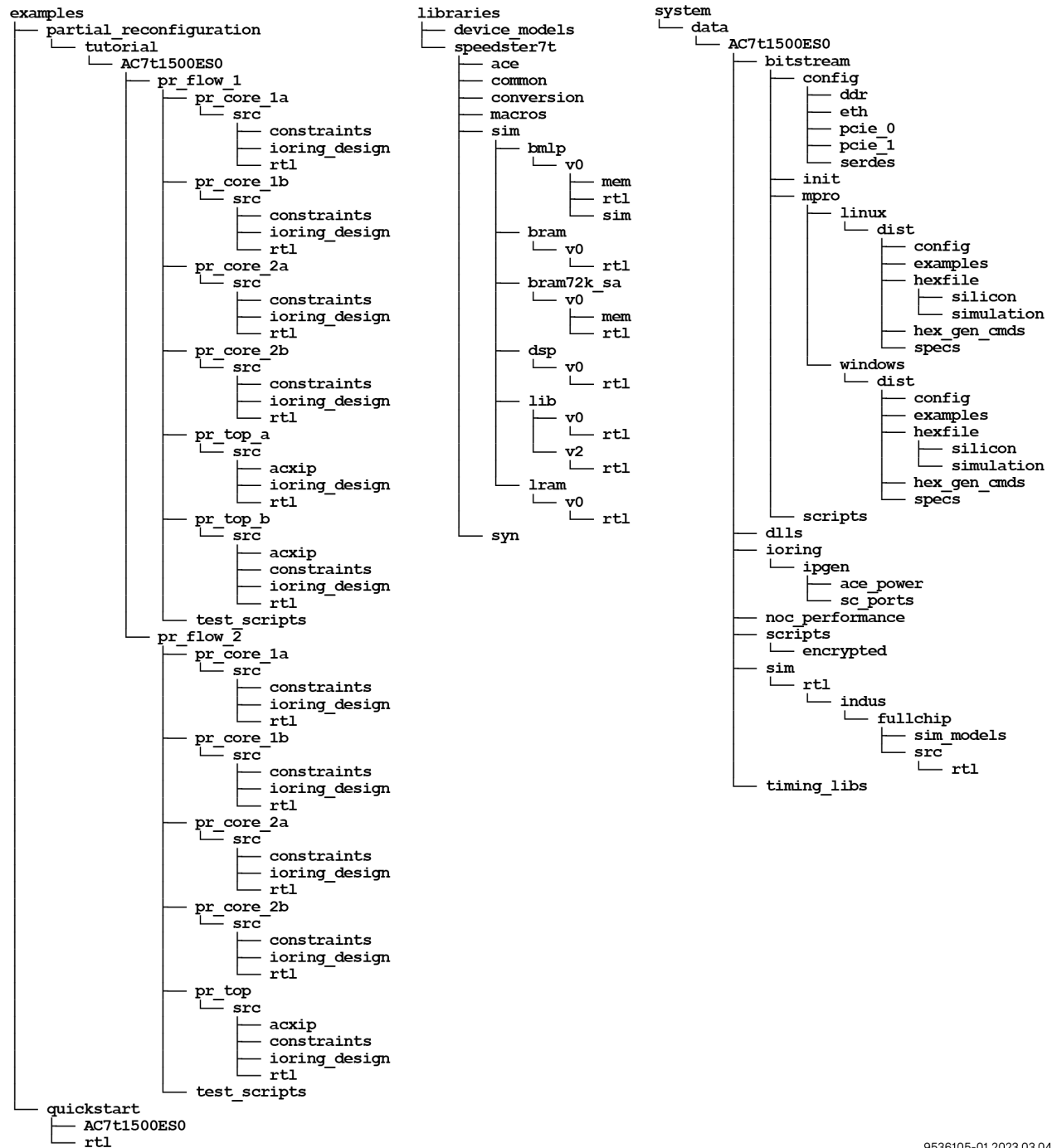
Figure 68: AC7t1500ES0 Overlay File Directory Structure
