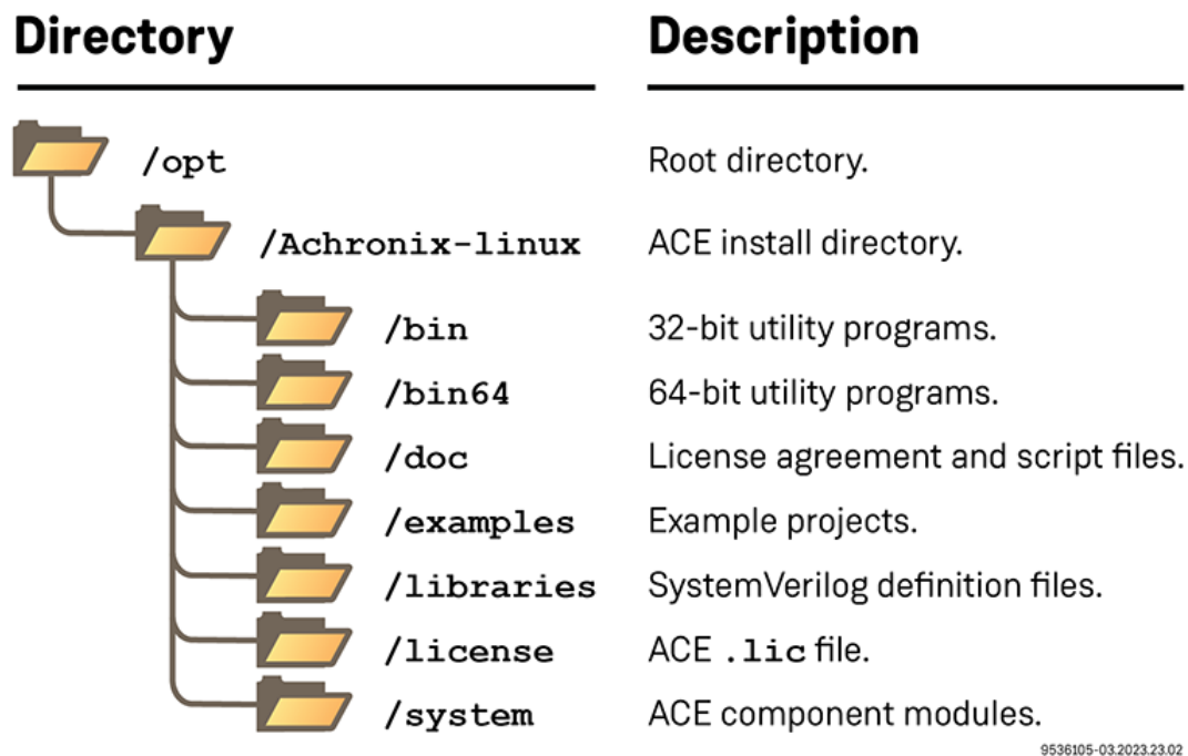
Figure 9: Ace Linux Directory Structure
