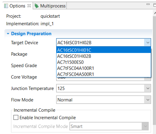
Figure 69: ACE Design Preparation Options Showing the Added Devices
